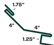
UNDER/OVER FLASHING
