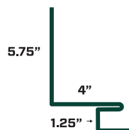
SIDE WALL FLASHING
