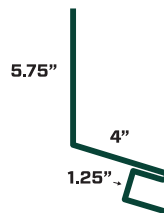
END WALL FLASHING
