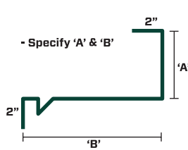
GABLE SOFFIT FASCIA
