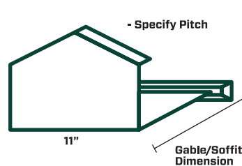
RIDGE BOX
