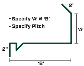
EAVE SOFFIT FASCIA
