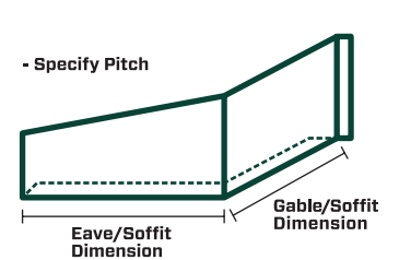
CORNER CAP
