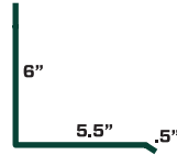
WALL FLASHING
