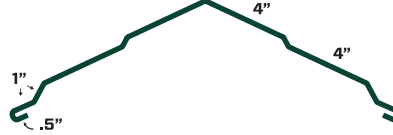
UNIVERSAL RIDGE CAP 9"
