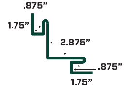
INSIDE CORNER WITH 'J'
