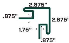
OUTSIDE CORNER WITH 'J'
