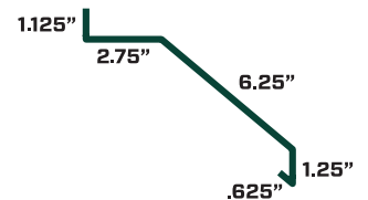
ROUND TRACK COVER
