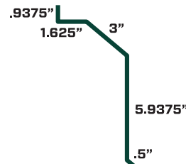
SQUARE TRACK COVER
