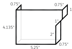
End Cap for 6" Eavestrough (ECET 6)
