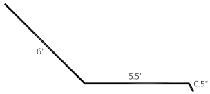
Under/Over Flashing (UOF)
