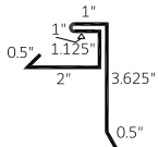
Flying Gable 1" (FG 1)
