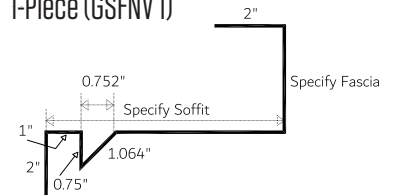
Gable Soffit/Fascia Non-Vented 1-Piece (GSFNV 1)
