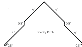
Ridge Cap R8 (RCR8)
