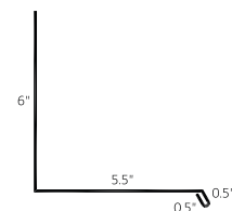
Side Wall Flashing with Hem (SWFH)
