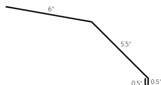
Gambrel Hip Cap with Hem (GHCH)
