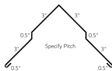
Ridge Cap R6 (RCR6)
