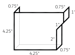
End Cap for 5" Eavestrough (ECET 5)
