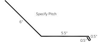
End Wall Flashing with Hem (EWFH)
