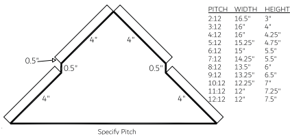
End Cap R8 (ECR8)
