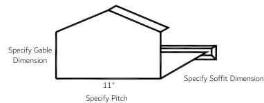
Ridge Box (RB)
