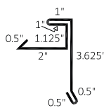
Flying Gable 1" with Hem (FGH 1)
