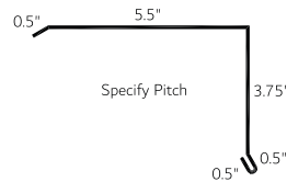
Cap Flashing 1" with Hem (CAPH 1)
