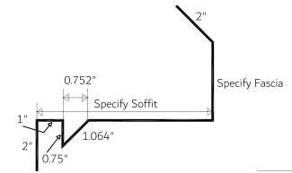
Eave Soffit/Fascia Vented 1-Piece (ESFV 1)
