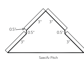
End Cap R6 (ECR6)
