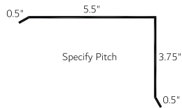
Cap Flashing 1" (CAP 1)
