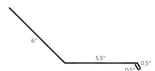
Under/Over Flashing with Hem (UOFH)
