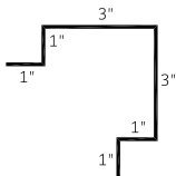
Outside Corner 1" (OC 1)
