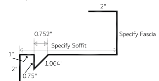
Gable Soffit/Fascia Vented 1-Piece (GSFV 1)
