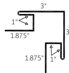
Outside Corner with 'J' 1" (OCJ 1)
