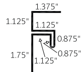
Wall Soffit Trim 1" (WST 1)
