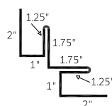
Inside Corner with 'J' 1" (ICJ 1)
