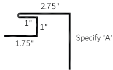
Jamb Flashing with 'J' 1" (JFJ 1)
