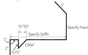
Eave Soffit/Fascia Vented 1-Piece (ESFV 1)
