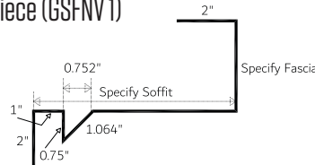
Gable Soffit/Fascia Non-Vented 1-Piece (GSFNV 1)
