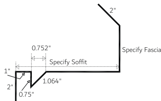
Eave Soffit/Fascia Non-Vented 1-Piece (ESFNV 1)
