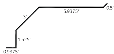
Square Track Cover (STC)
