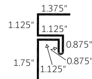
Wall Soffit Trim 1" (WST 1)
