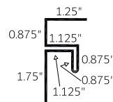
Wall Ceiling Trim 1" (WCT 1)
