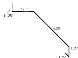
Round Track Cover (RTC)
