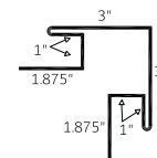
Outside Corner with 'J' 1" (OCJ 1)
