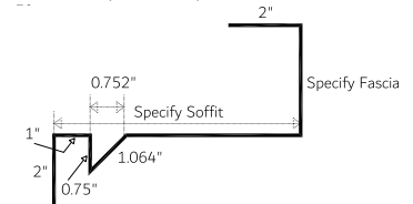
Gable Soffit/Fascia Non-Vented 1-Piece (GSFNV 1)
