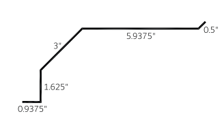
Square Track Cover (STC)
