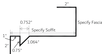
Gable Soffit/Fascia Vented 1-Piece (GSFV 1)
