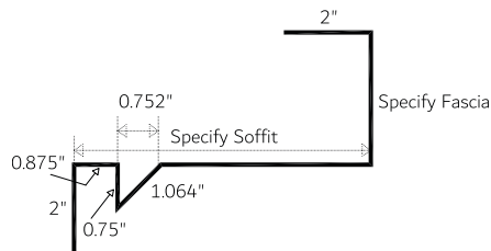
Gable Soffit/Fascia Vented 1-Piece (GSFV 0.75)
