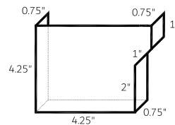
Fascia 6" (FAS 6)
