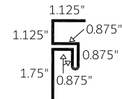
Wall Soffit Trim 3/4" (WST 0.75)
