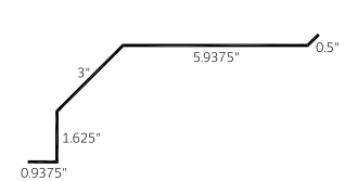
Square Track Cover (STC)
