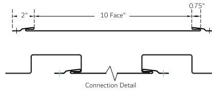
Coupler Side (COUS 12)
