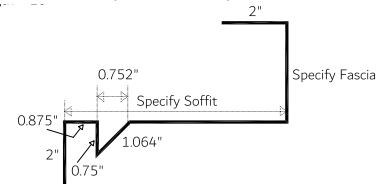
Gable Soffit/Fascia Non-Vented 1-Piece (GSFNV 0.75)
