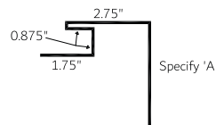
Jamb Flashing with 'J' 3/4" (JFJ 0.75)
