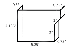
Fascia 8" (FAS 8)
