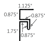
Wall Ceiling Trim 3/4" (WCT 0.75)
