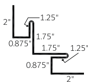
Inside Corner with 'J' 3/4" (ICJ 0.75)
