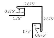
Outside Corner with 'J' 3/4" (OCJ 0.75)
