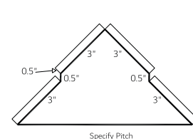
End Cap R6 (ECR6)
