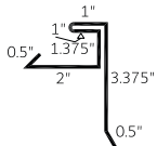
Flying Gable 1-1/4" (FG 1.25)
