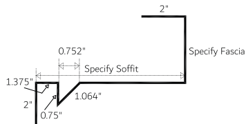
Gable Soffit/Fascia Vented 1-Piece (GSFV 1.25)
