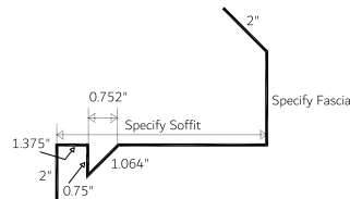
Eave Soffit/Fascia Non-Vented 1-Piece (ESFNV 1.25)
