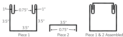
Downspout 2-piece (DS)
