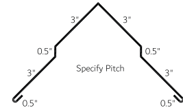
Ridge Cap R6 (RCR6)
