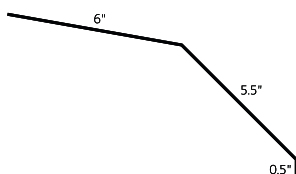
Gambrel Hip Cap (GHC)
