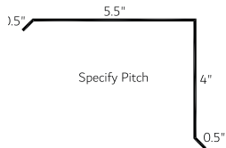
Cap Flashing 1-1/4" (CAP 1.25)
