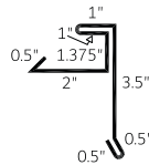
Flying Gable 1-1/4" with Hem (FGH 1.25)
