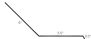
Under/Over Flashing (UOF)
