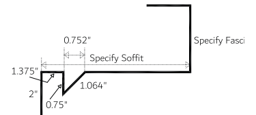
Gable Soffit/Fascia Non-Vented 1-Piece (GSFNV 1.25)
