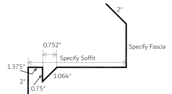
Eave Soffit/Fascia Vented 1-Piece (ESFV 1.25)
