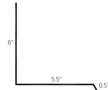
Side Wall Flashing (SWF)
