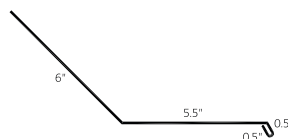
Under/Over Flashing with Hem (UOFH)
