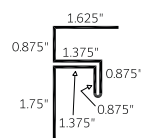
Wall Ceiling Trim 1-1/4" (WCT 1.25)
