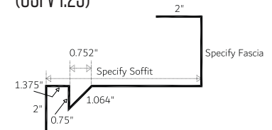
Gable Soffit/Fascia Vented 1-Piece (GSFV 1.25)
