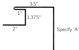
Jamb Flashing with 'J' 1-1/4" (JFJ 1.25)
