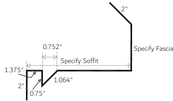
Eave Soffit/Fascia Non-Vented 1-Piece (ESFNV 1.25)
