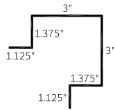
Outside Corner 1-1/4" (OC 1.25)
