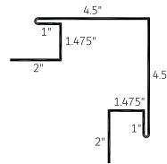
Outside Corner with 'J' 1-1/4" (OCJ 1.25)
