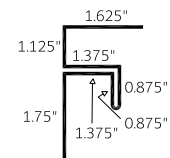
Wall Soffit Trim 1-1/4" (WST 1.25)
