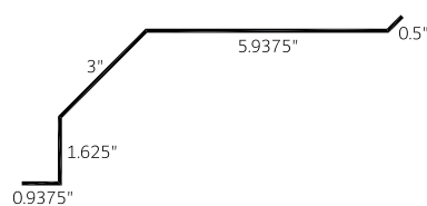
Square Track Cover (STC)
