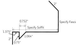
Eave Soffit/Fascia Vented 1-Piece (ESFV 1.25)
