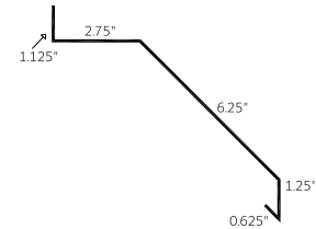
Round Track Cover (RTC)
