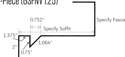
Gable Soffit/Fascia Non-Vented 1-Piece (GSFNV 1.25)
