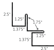
Inside Corner with 'J' 1-1/4" (ICJ 1.25)
