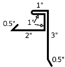
Gable Soffit/Fascia Vented 1-Piece (GSFV 0.75)
