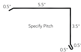
Cap Flashing 3/4" with Hem (CAPH 0.75)
