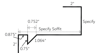
Gable Soffit/Fascia Non-Vented 1-Piece (GSFNV 0.75)
