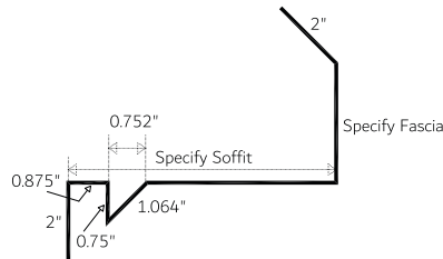
Eave Soffit/Fascia Non-Vented 1-Piece (ESFNV 0.75)
