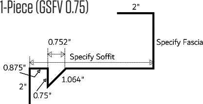
Gable Soffit/Fascia Vented 1-Piece (GSFV 0.75)
