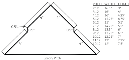
End Cap R8 (ECR8)
