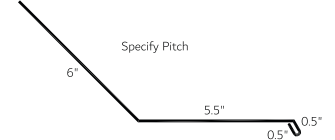
End Wall Flashing with Hem (EWFH)
