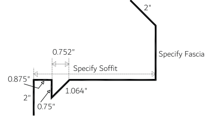
Eave Soffit/Fascia Vented 1-Piece (ESFV 0.75)
