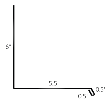
Side Wall Flashing with Hem (SWFH)
