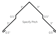
Ridge Cap R6 (RCR6)
