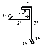
Flying Gable 3/4" with Hem (FGH 0.75)
