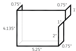
End Cap for 6" Eavestrough (ECET 6)
