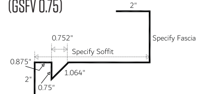
Gable Soffit/Fascia Vented 1-Piece (GSFV 0.75)
