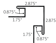
Outside Corner with 'J' 3/4" (OCJ 0.75)
