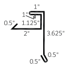
Flying Gable 1" with Hem (FGH 1)
