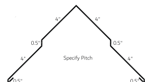
Ridge Cap R8 (RCR8)
