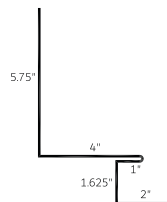
Legacy Side Wall Flashing 1.5" (LSWF 1.5)
