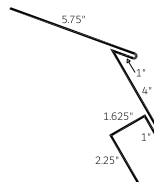
Legacy Gambrel Hip Cap 1.5" (LGHC 1.5)
