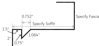
Gable Soffit/Fascia Vented 1-Piece (GSFV 1.5)
