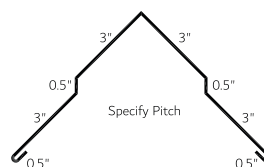
Ridge Cap R6 (RCR6)
