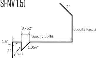
Eave Soffit/Fascia Non-Vented 1-Piece (ESFNV 1.5)
