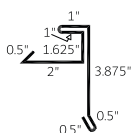
Flying Gable 1.5" with Hem (FGH 1.5)
