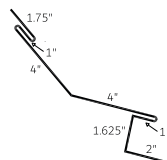
Legacy Gambrel Hip Cap 1.5" (LGHC 1.5)
