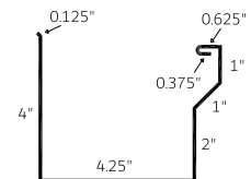
End Cap for 5" Eavestrough (ECET 5)
