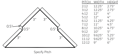
End Cap R6 (ECR6)
