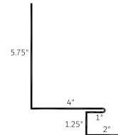
Legacy Side Wall Flashing 1" (LSWF 1)
