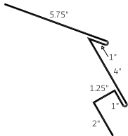
Legacy Gambrel Hip Cap 1" (LGHC 1)
