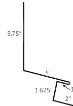
Legacy End Wall Flashing 1.5" (LEWF 1.5)
