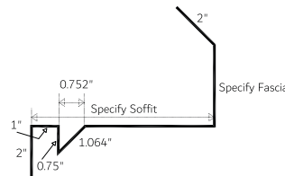
Eave Soffit/Fascia Vented 1-Piece (ESFV 1)
