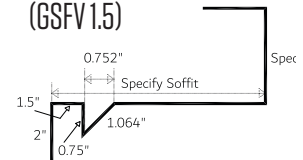
Gable Soffit/Fascia Vented 1-Piece (GSFV 1.5)
