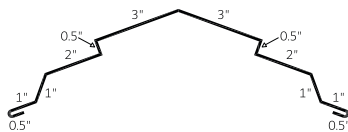
Legacy Ridge Cap Universal 6" (LRCU6)
