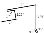
Legacy Cap Flashing 1" (LCAP 1)
