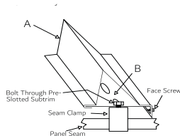
Legacy Snow Stop Subtrim Galvanized 18ga (LSNOSUB 18)
