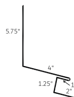
Legacy End Wall Flashing 1" (LEWF 1)
