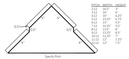
End Cap R8 (ECR8)
