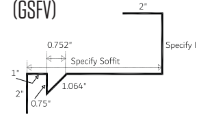
Gable Soffit/Fascia Vented 1-Piece (GSFV)
