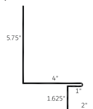
Legacy Side Wall Flashing 1.5" (LSWF 1.5)
