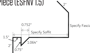
Eave Soffit/Fascia Non-Vented 1-Piece (ESFNV 1.5)
