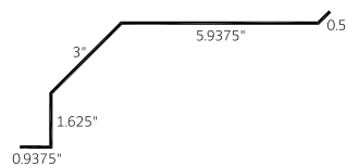
Square Track Cover (STC)
