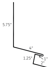
Legacy End Wall Flashing 1" (LEWF 1)
