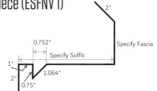
Eave Soffit/Fascia Non-Vented 1-Piece (ESFNV 1)
