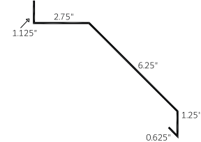
Round Track Cover (RTC)
