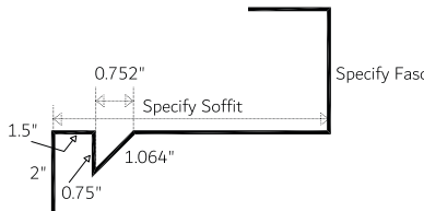
Gable Soffit/Fascia Vented 1-Piece (GSFV 1.5)
