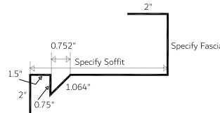
Gable Soffit/Fascia Non-Vented 1-Piece (GSFNV 1.5)
