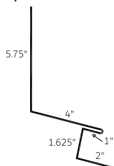
Legacy End Wall Flashing 1.5" (LEWF 1.5)
