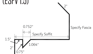
Eave Soffit/Fascia Vented 1-Piece (ESFV 1.5)
