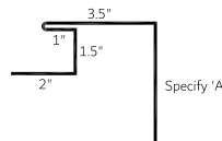
Jamb Flashing with 'J' 1" (JFJ 1)
