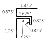
Wall Ceiling Trim 1-1/2" (WCT 1.5)
