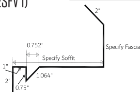
Eave Soffit/Fascia Vented 1-Piece (ESFV 1)
