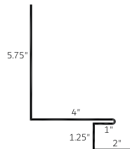
Legacy Side Wall Flashing 1" (LSWF 1)
