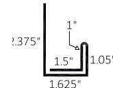
J-Trim Commercial 1-1/2" (JTC 1.5)
