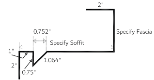
Gable Soffit/Fascia Non-Vented 1-Piece (GSFNV 1)
