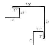
Outside Corner with 'J' 1-1/2" (OCJ 1.5)
