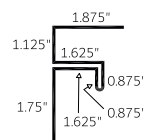
Wall Soffit Trim 1-1/2" (WST 1.5)
