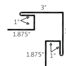
Outside Corner with 'J' 1" (OCJ 1)
