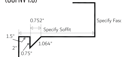
Gable Soffit/Fascia Non-Vented 1-Piece (GSFNV 1.5)
