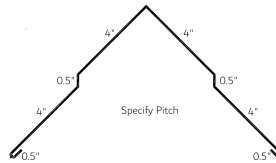
Ridge Cap R8 (RCR8)
