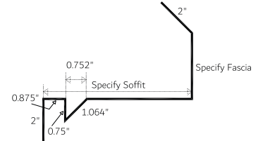
Eave Soffit/Fascia Vented 1-Piece (ESFV 0.75)
