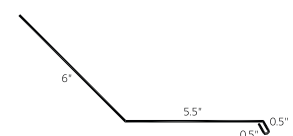
Under/Over Flashing with Hem (UOFH)
