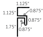
Wall Soffit Trim 3/4" (WST 0.75)
