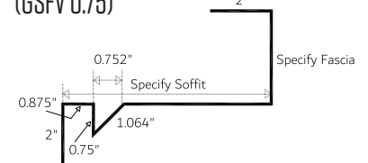
Gable Soffit/Fascia Vented 1-Piece (GSFV 0.75)
