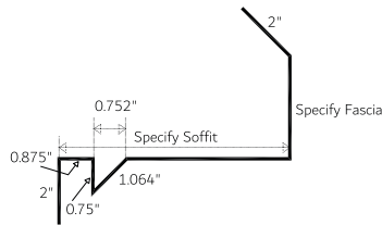
Eave Soffit/Fascia Non-Vented 1-Piece (ESFNV 0.75)
