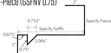
Gable Soffit/Fascia Non-Vented 1-Piece (GSFNV 0.75)
