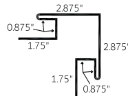
Outside Corner with 'J' 3/4" (OCJ 0.75)
