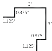
Outside Corner 3/4" (OC 0.75)
