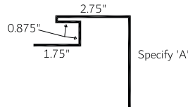
Jamb Flashing with 'J' 3/4" (JFJ 0.75)
