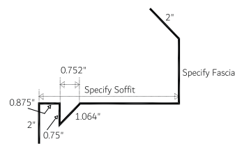
Eave Soffit/Fascia Vented 1-Piece (ESFV 0.75)
