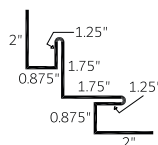
Inside Corner with 'J' 3/4" (ICJ 0.75)
