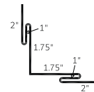
Inside Corner with 'J' 1/8" (ICJ 0.125)
