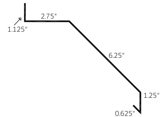
Round Track Cover (RTC)
