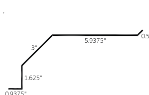
Square Track Cover (STC)
